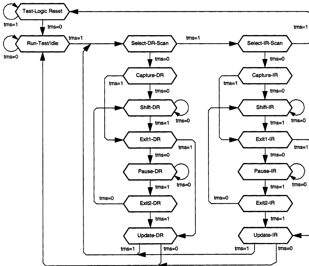
Figure 52: Test Access Port (TAP) Controller State Transitions
