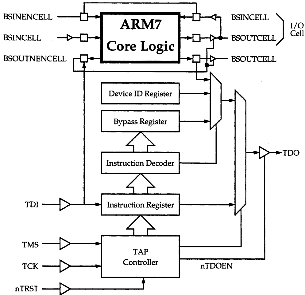
Figure 53: Boundary Scan Block Diagram
