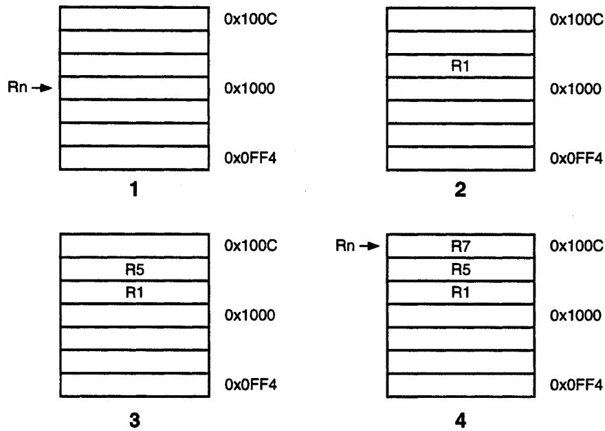
Figure 23: Pre-increment addressing
