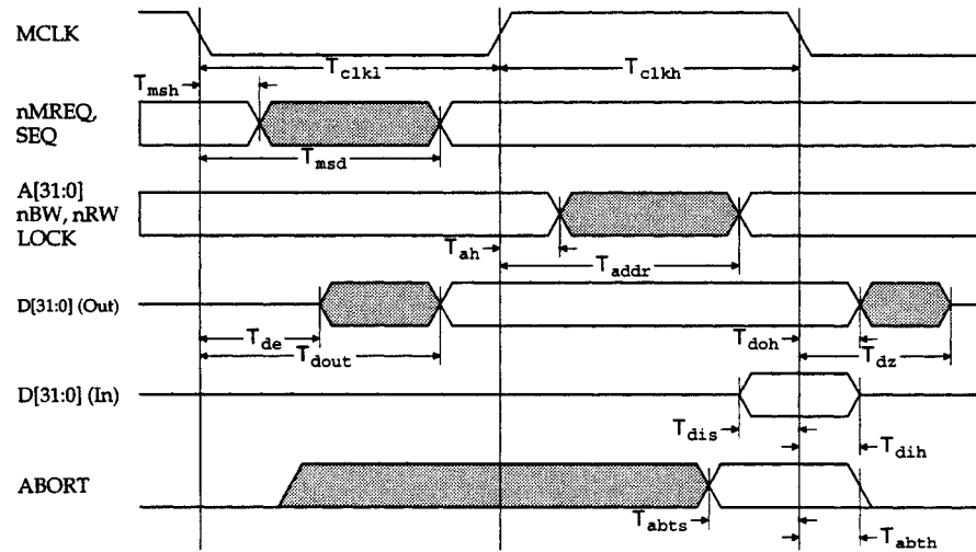
Figure 59: ARM710 Main Bus Timing
