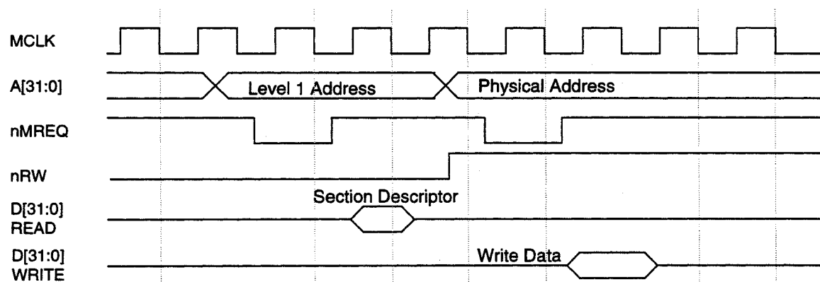
Figure 49: Translation Table-walking Sequence (write) For Section
