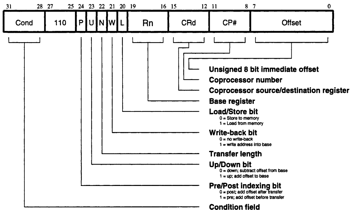
Figure 29: Coprocessor Data Transfer Instructions
