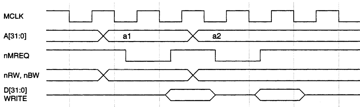
Figure 46: Two Word Non-Sequential Buffered Writes
