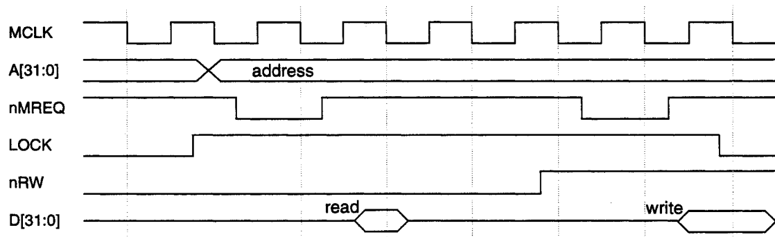
Figure 50: Read - Locked - Write
