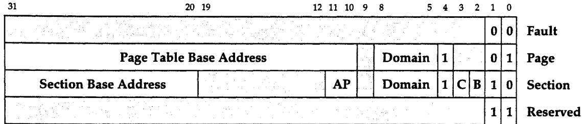
Figure 36: Level One Descriptors
