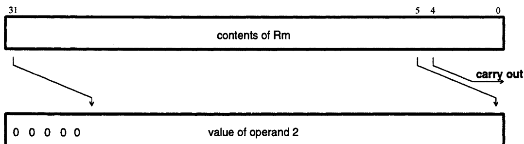
Figure 13: Logical Shift Right
