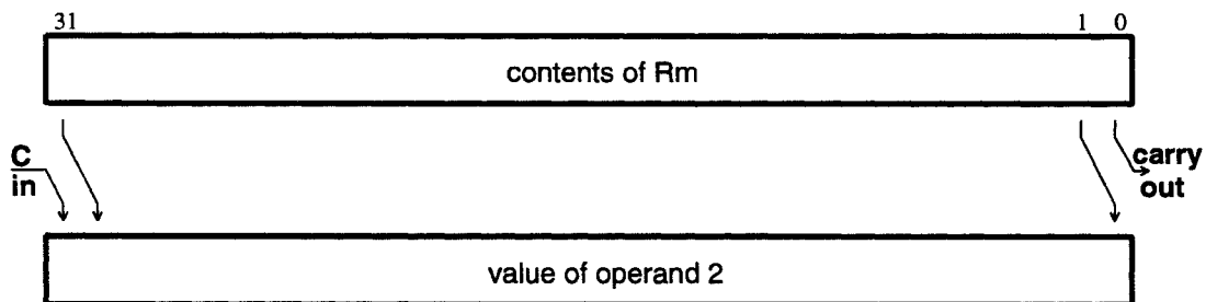
Figure 16: Rotate Right Extended
