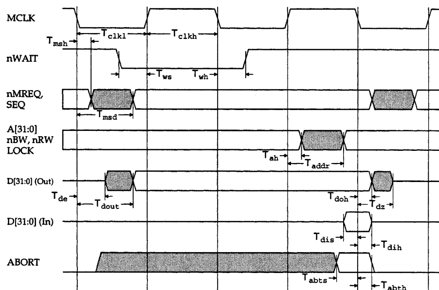
Figure 61: ARM710 nWAIT Timing
