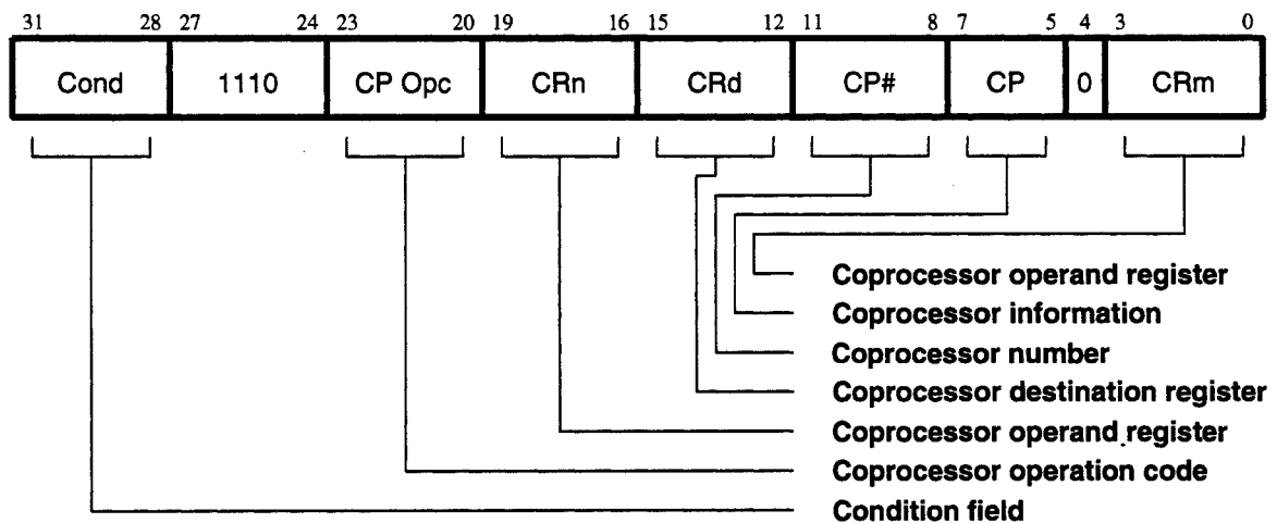
Figure 28: Coprocessor Data Operation Instruction
