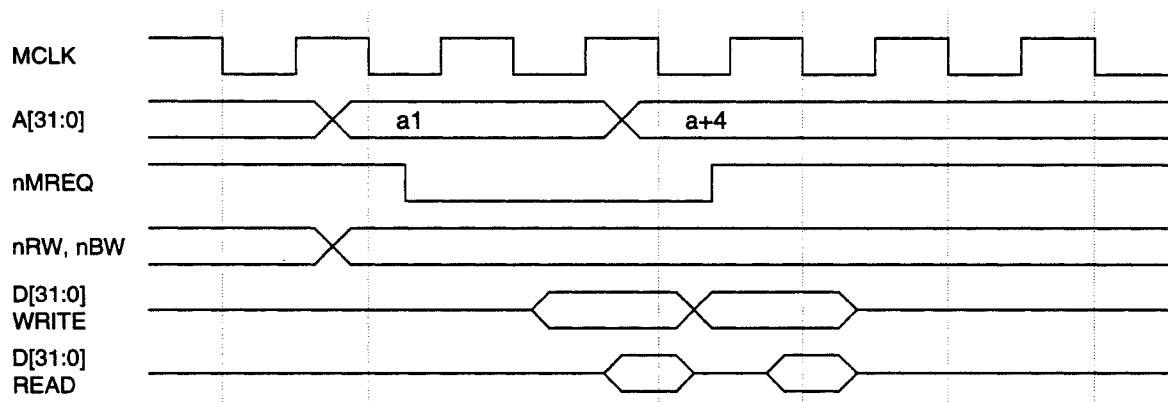
Figure 44: Two Word Sequential Read or Write
