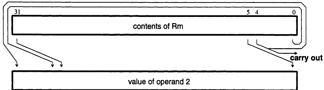
Figure 15: Rotate Right
