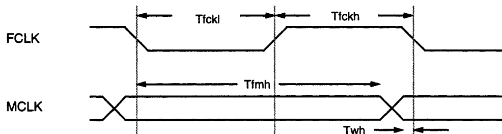
Figure 57: Clock Timing Relationship
