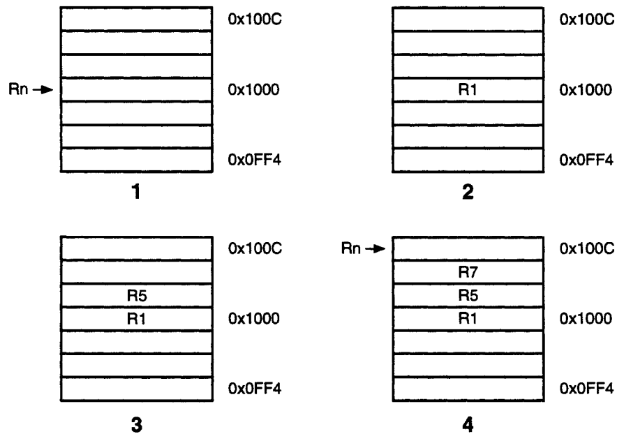
Figure 22: Post-increment addressing
