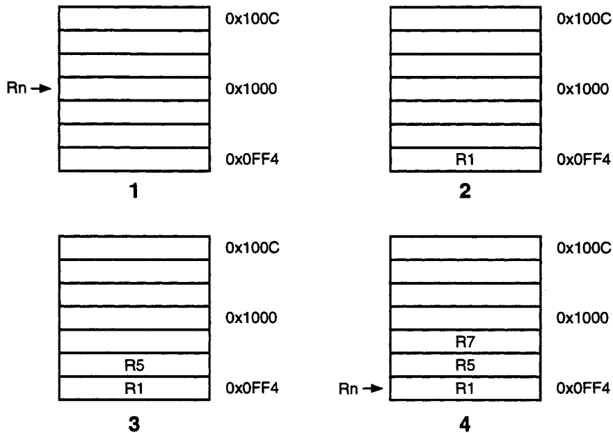
Figure 25: Pre-decrement addressing
