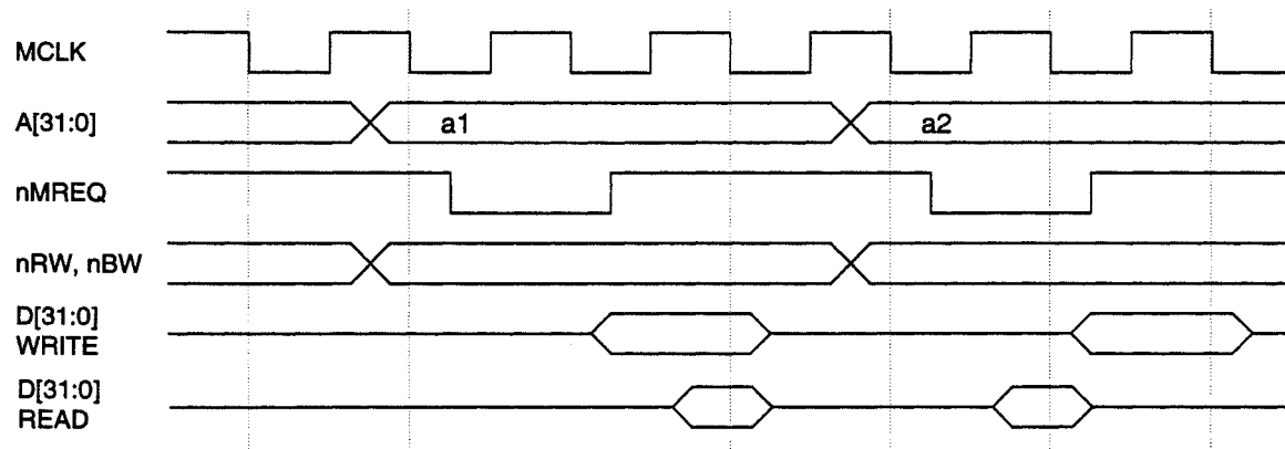
Figure 45: Two Word Non-Sequential Unbuffered accesses
