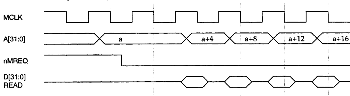
Figure 47: Linefetch
