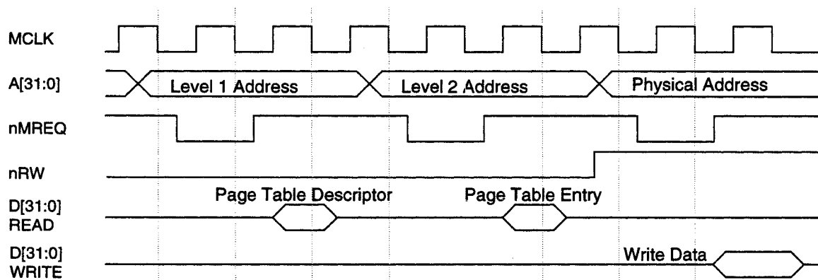
Figure 48: Translation Table-walking Sequence (write) For Page
