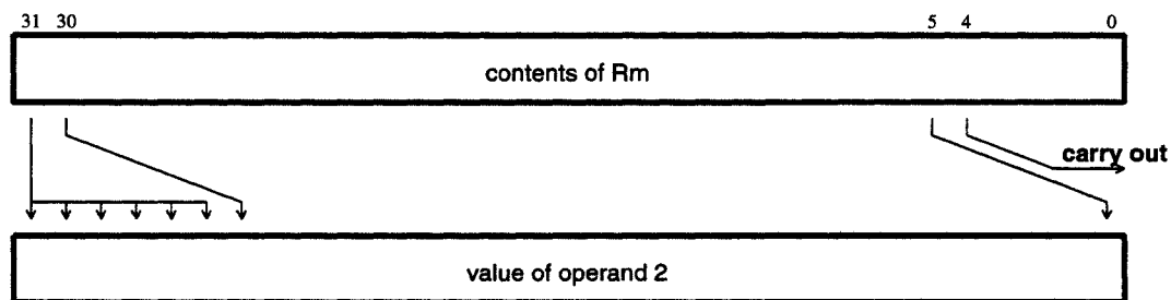
Figure 14: Arithmetic Shift Right
