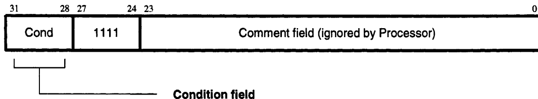
Figure 27: Software Interrupt Instruction
