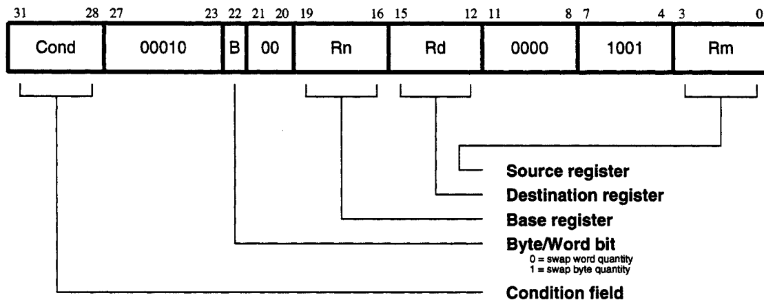
Figure 26: Swap Instruction
