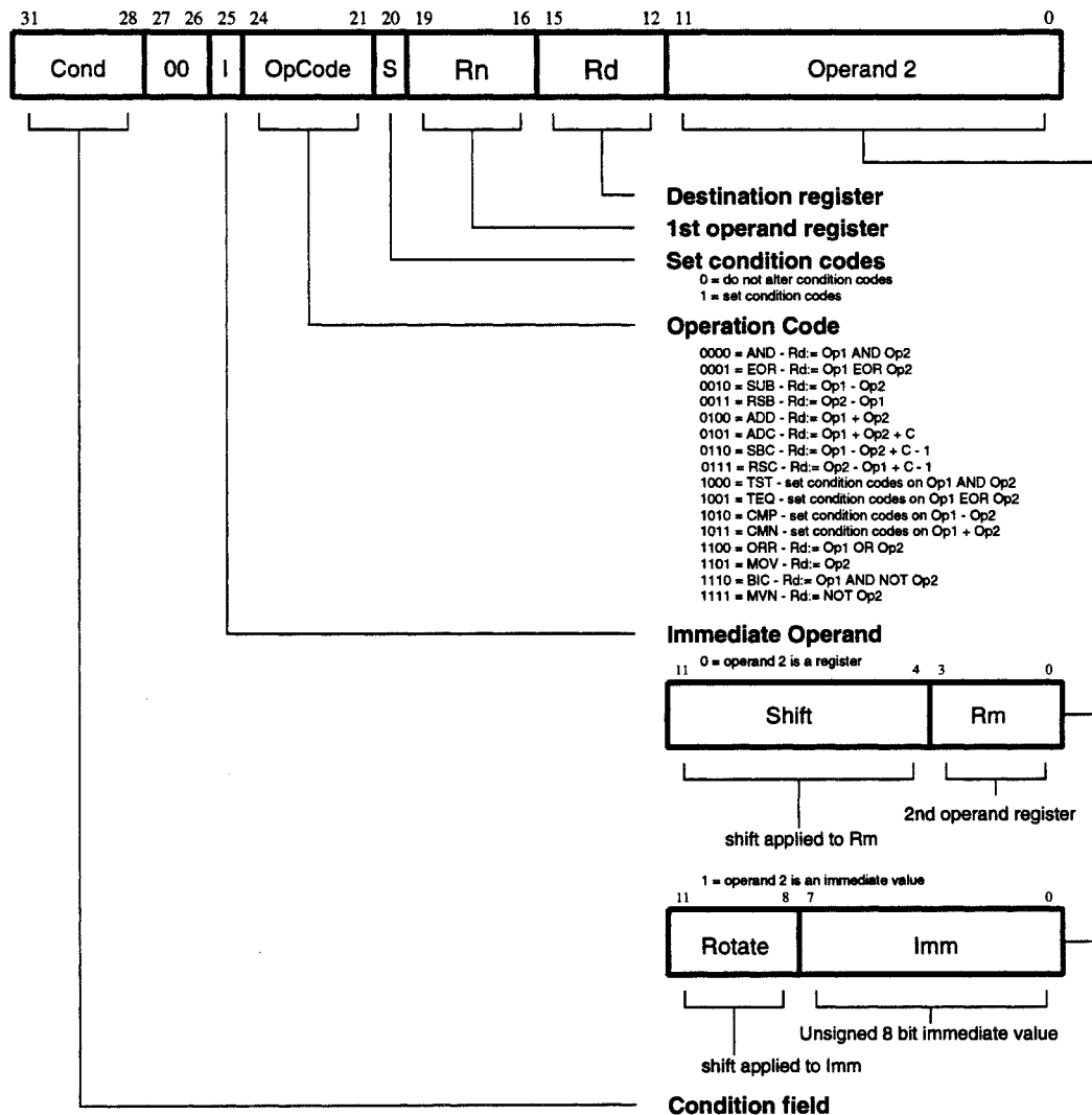
Figure 10: Data Processing Instructions
