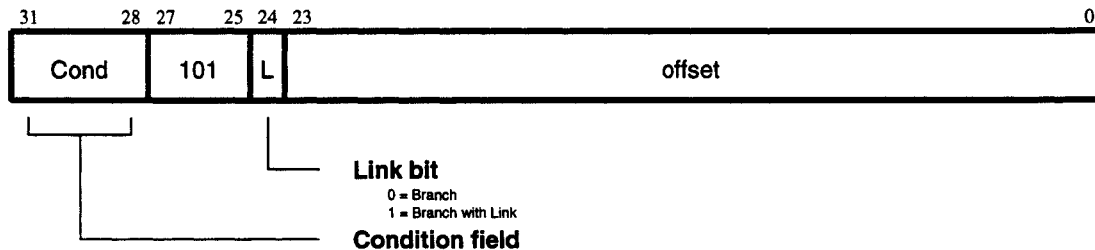
Figure 9: Branch Instructions
