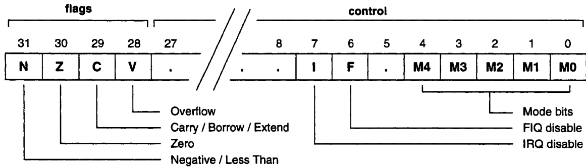
Figure 6: Format of the Program Status Registers (PSRs)
