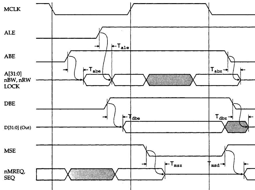
Figure 60: ARM710 Bus Enable Timing
