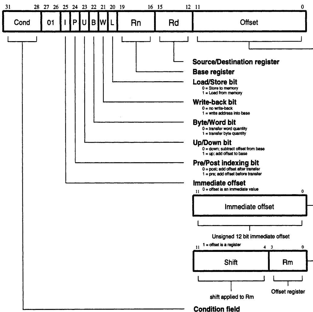
Figure 19: Single Data Transfer Instructions
