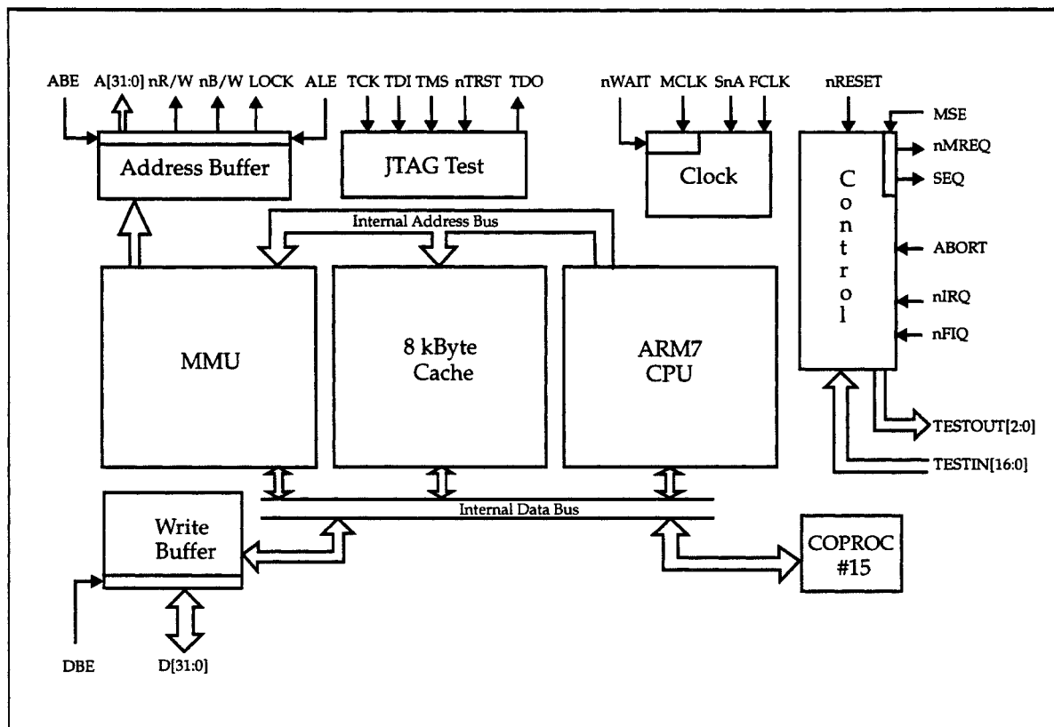
Figure 1: ARM710 Block Diagram
