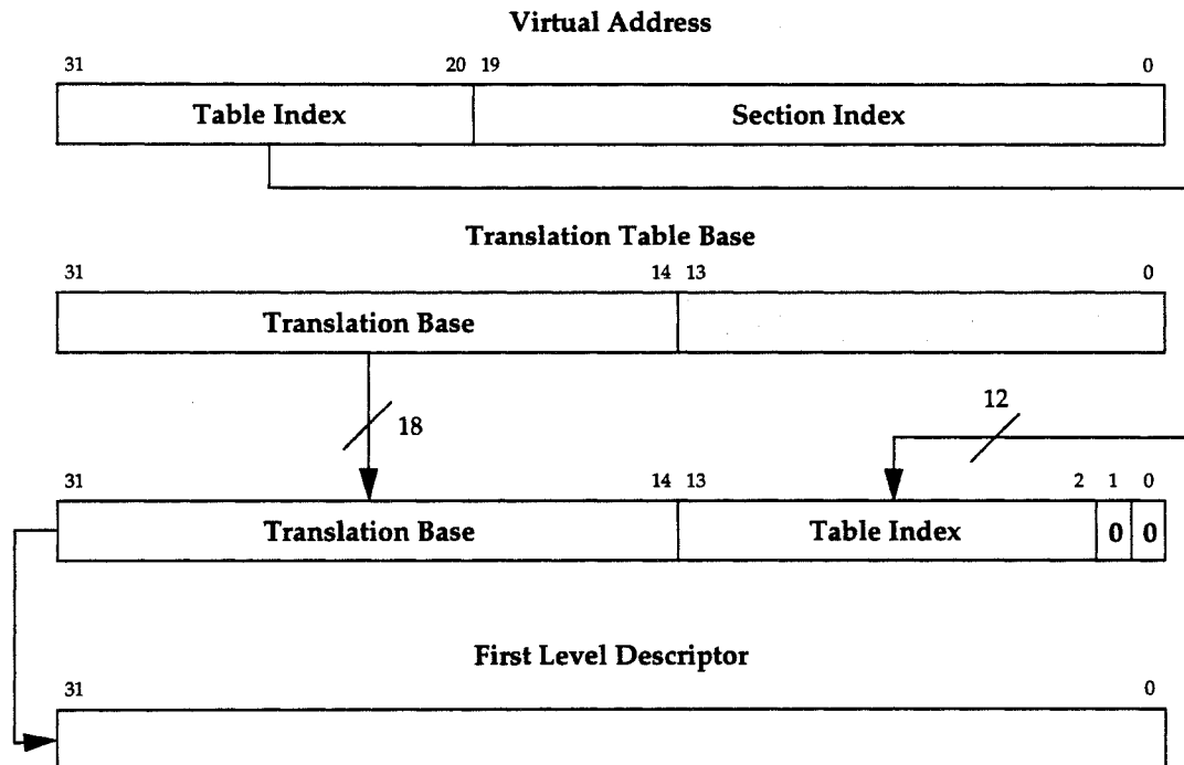
Figure 35: Accessing the Translation Table First Level Descriptors
