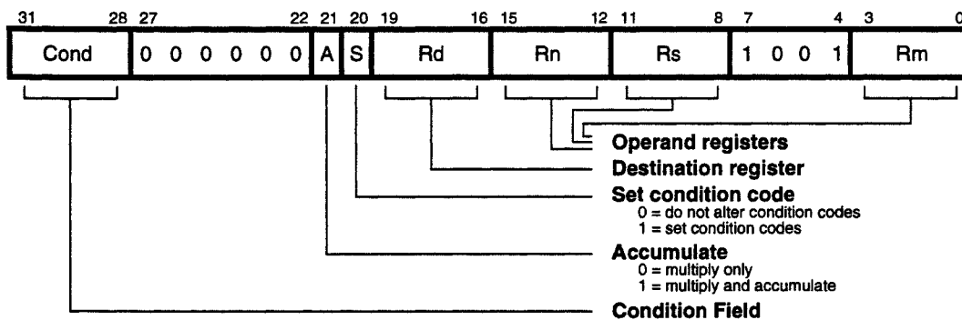
Figure 18: Multiply Instructions
