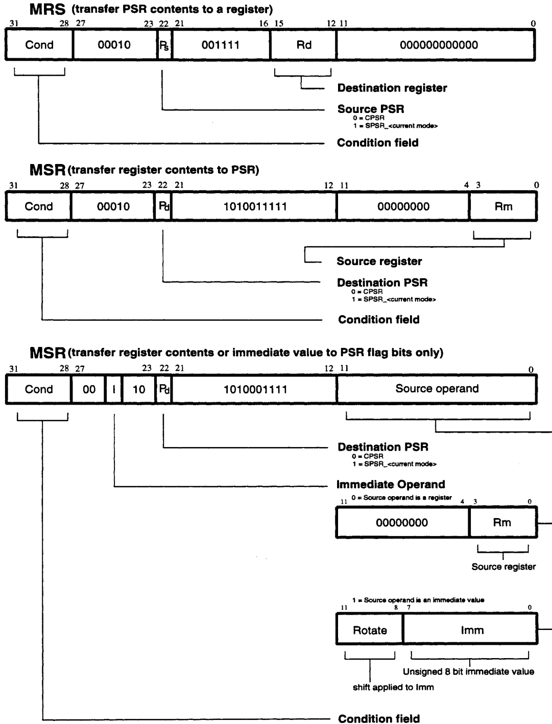
Figure 17: PSR Transfer
