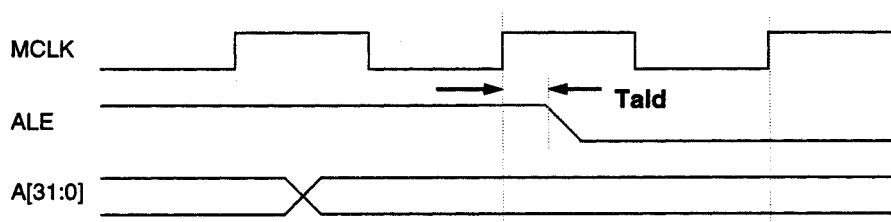
Figure 58: Tald Measurement
