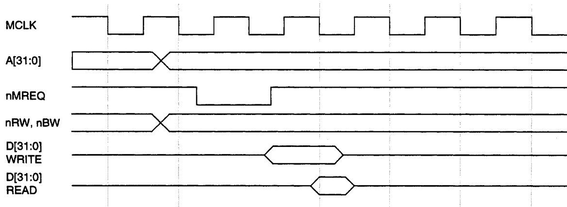
Figure 43: One word Read or Write
