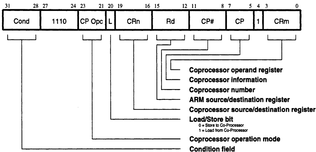
Figure 30: Coprocessor Register Transfer Instructions
